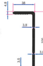
100x38 mm PERVAZ
