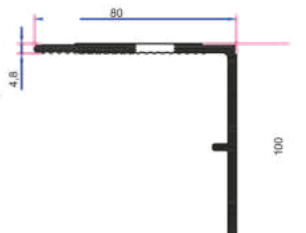
80x100 mm PERVAZ
