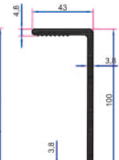
100x43x18 mm PERVAZ
