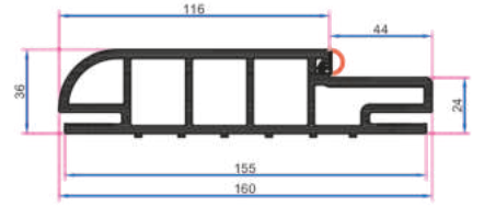
OVAL 160mm KAPI KASA
