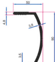
50x90 mm OVAL PERVAZ
