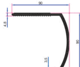
90x90 mm OVAL PERVAZ
